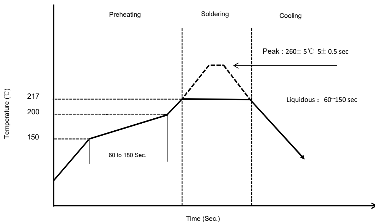
Figure 1. Re-flow Soldering
