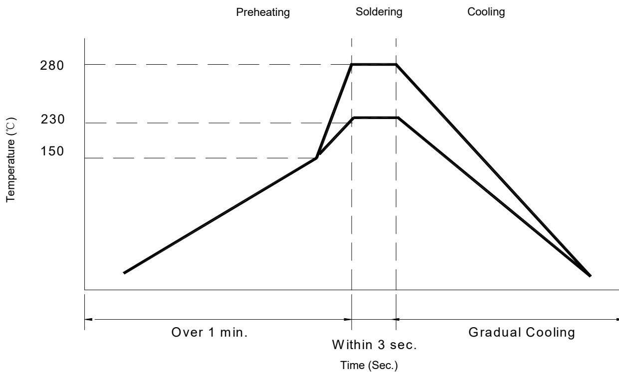
Figure 2. Hand Soldering
